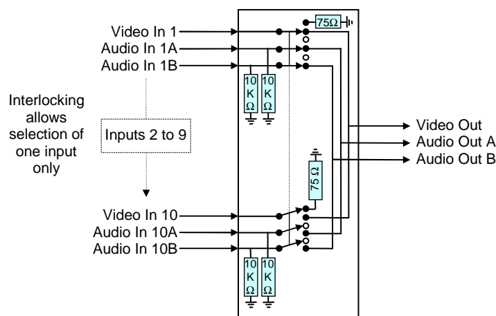
BLOCK DIAGRAM AMS-1000 SIGNAL PATH
