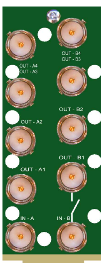
Optional Relay Bypass Rear Assembly (IRT-6010RL-ZDA)
